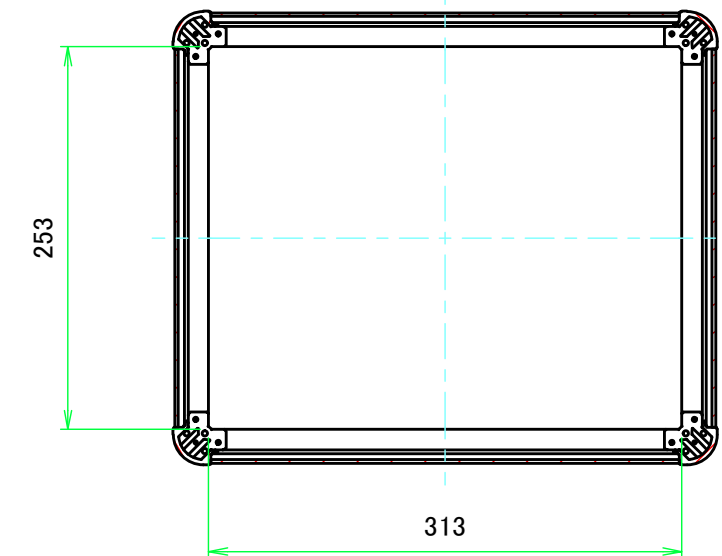
C-C (1:5)
