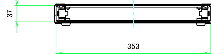
B-B (1:5)
